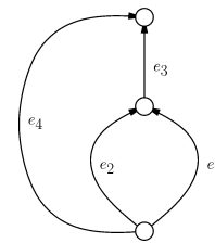
Figure 2: An example of a DAG that does not admit a shortest path protocol that operates in a single round under the shared and routing protocols.
